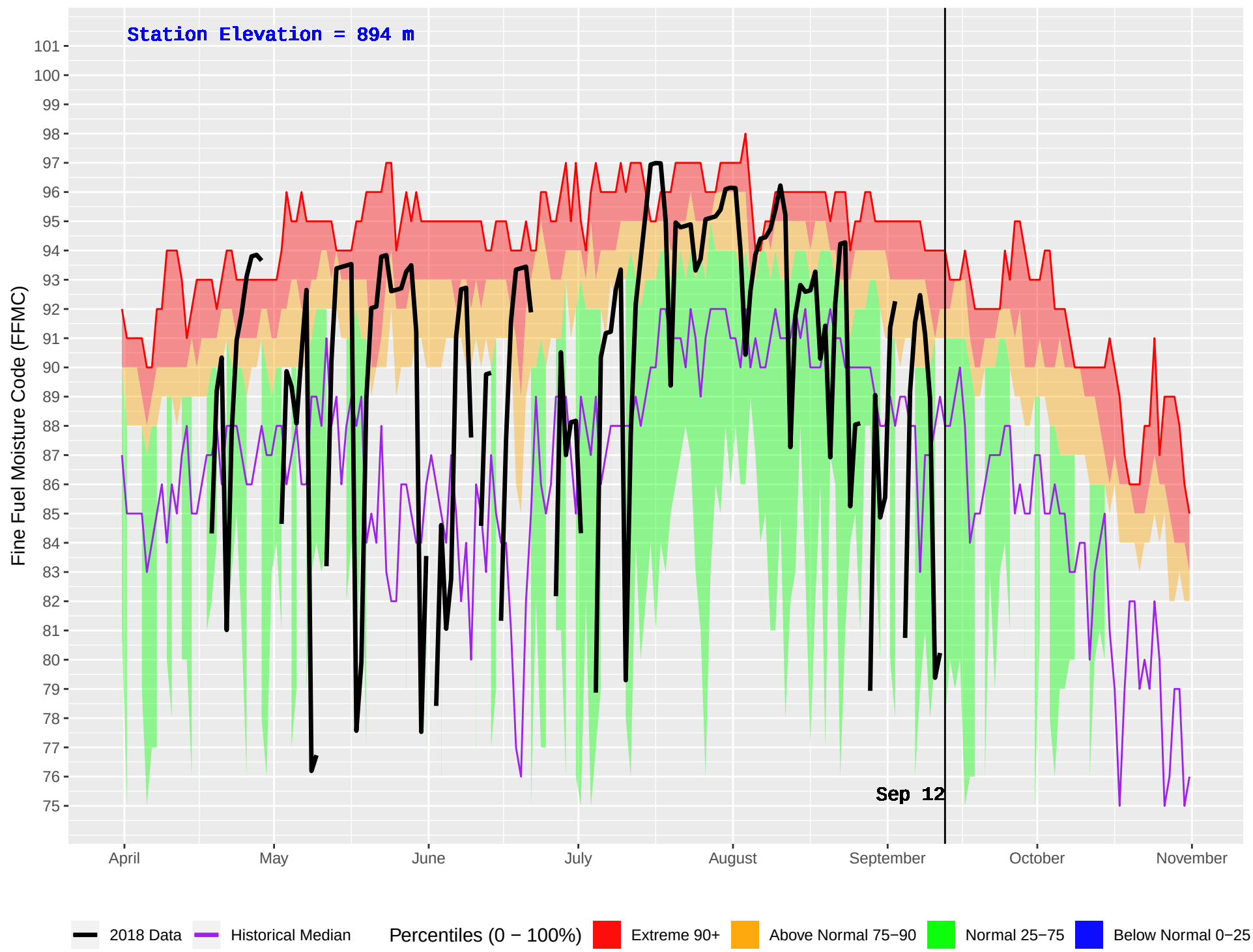
TOBY HUB (417) : Historical (1986–2016) and Current (2018) Daily Fine Fuel Moisture Code (FFMC)
